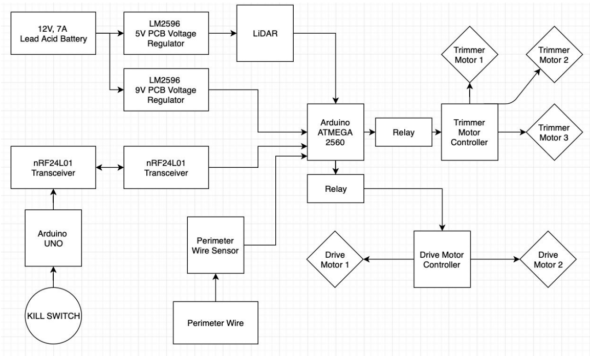
Figure 67: Final Block Diagram
