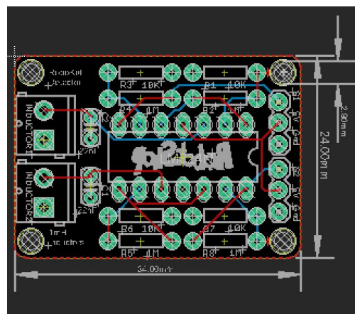
Figure 60: Sensor PCB
