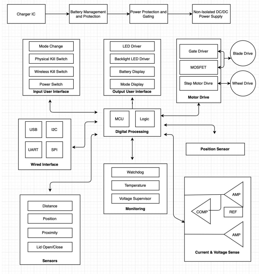
Figure 49: MCU Layout
