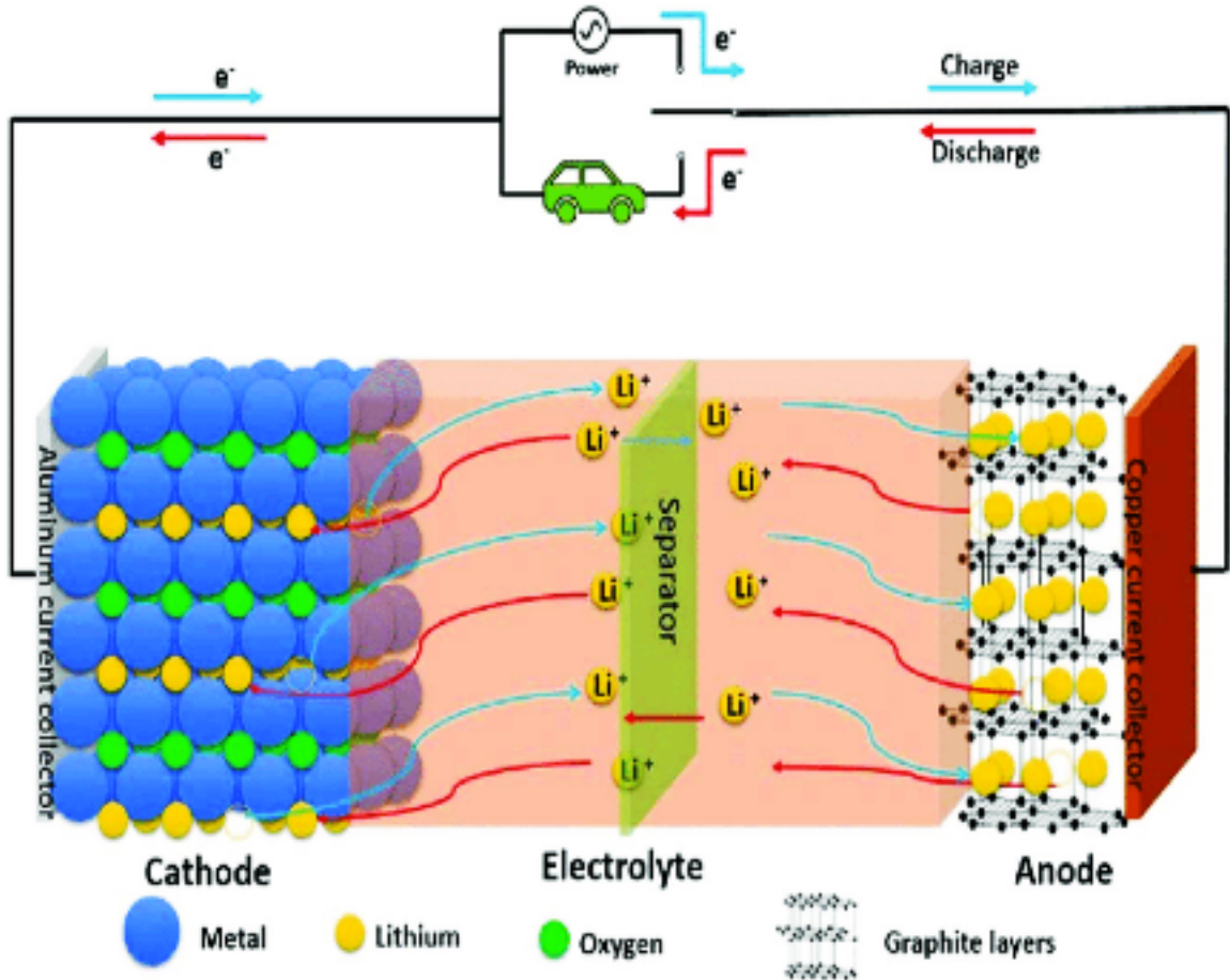
Figure 22: Lithium-Ion Schematic
