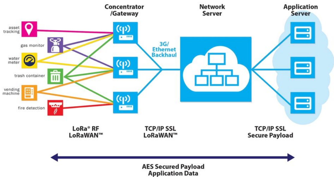
Figure 17: LoraWAN Web
