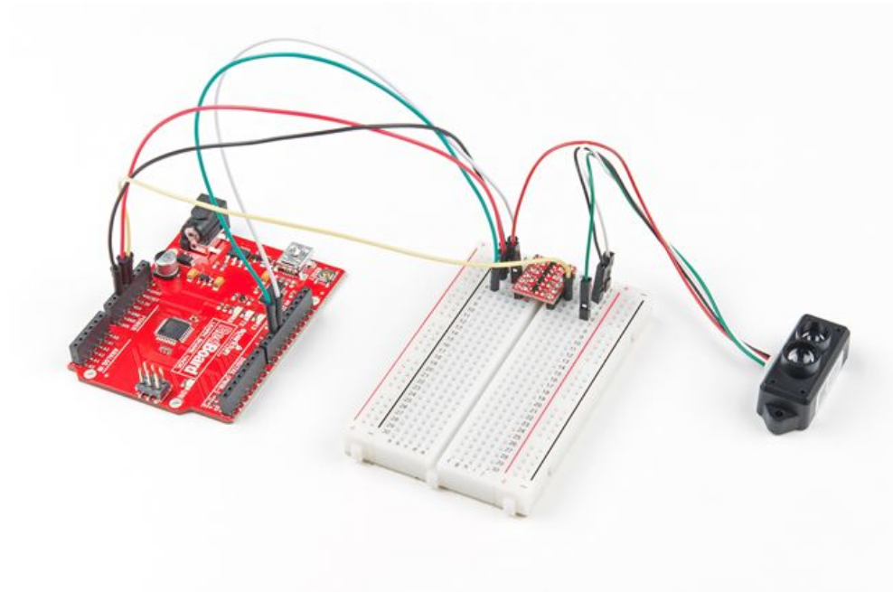
Figure 28: TF Mini LiDar hooked up to microcontroller w/ logic converter
