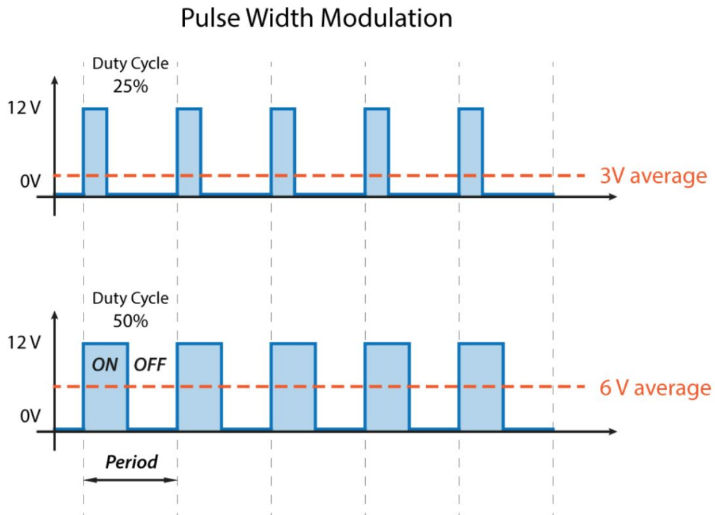
Figure 19: PWM Speed Control
