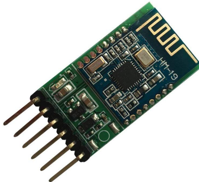
Figure 16: DSD TECH HM-19 Bluetooth 5.0 BLE Module with CC2640R2F Chip for Arduino and DIY
