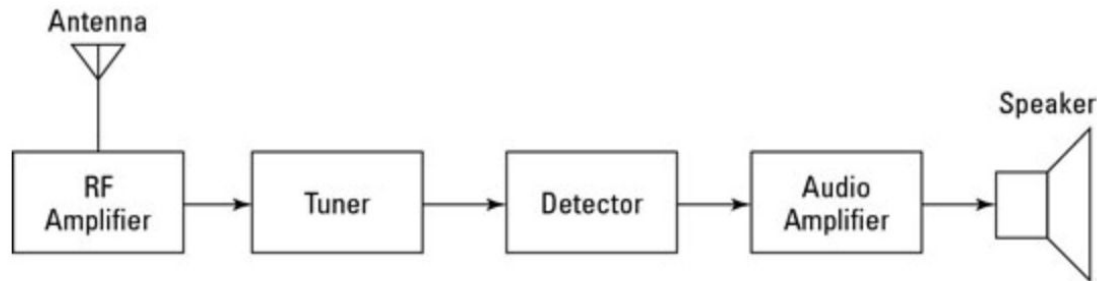
Figure 14: Receiver Diagram
