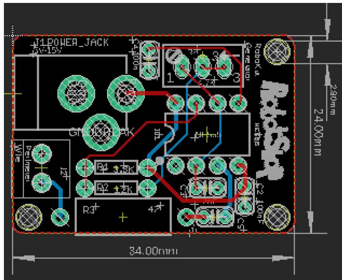
Figure 57: Wire Generator PCB
