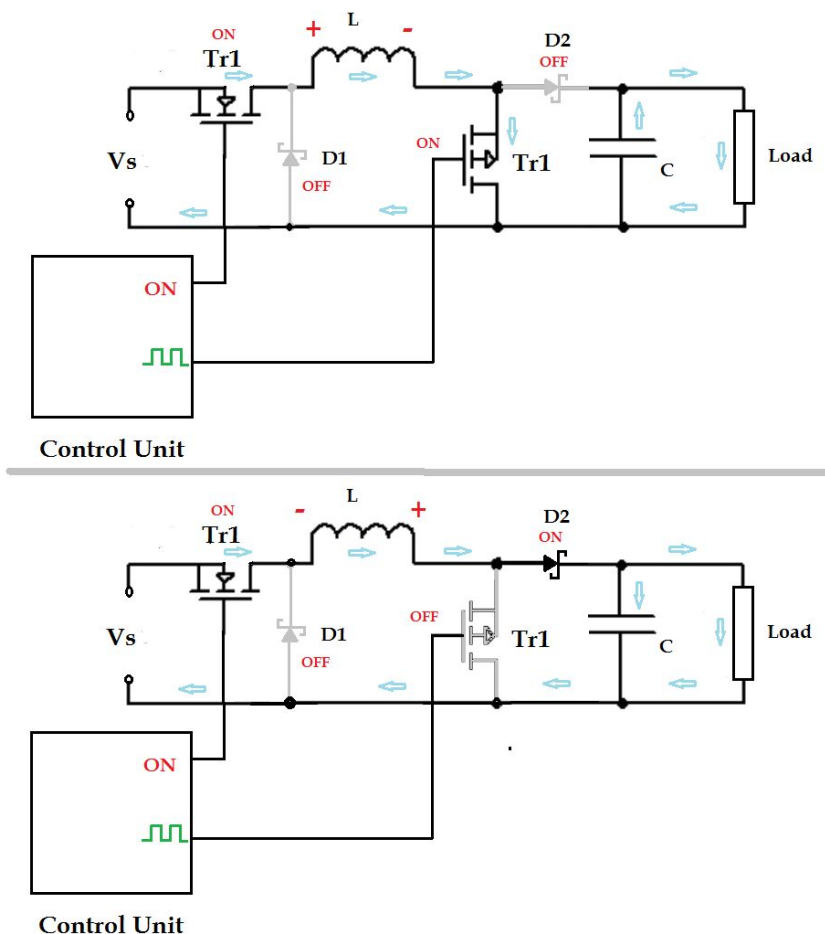
Figure 11: Buck mode of converter
