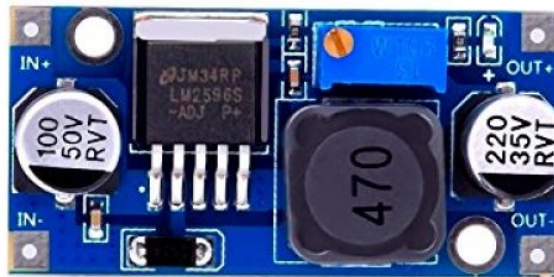
Figure 20: LM2596S Chip
