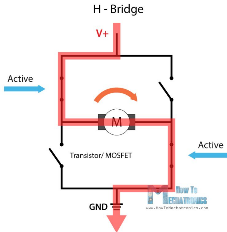
Figure 18: H-Bridge Motor Diagram
