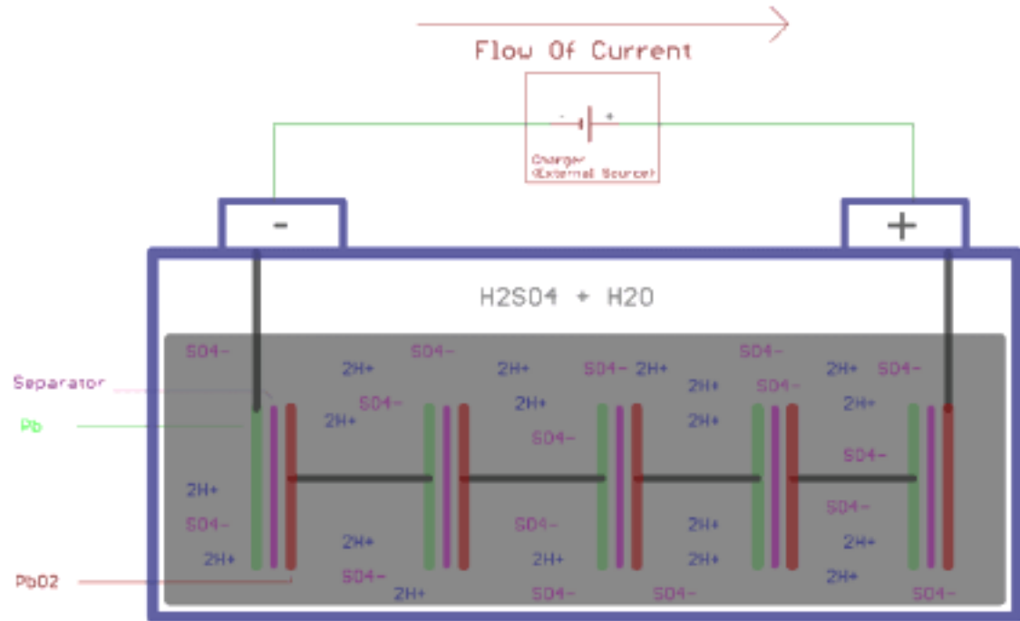
Figure 24: Lead-Acid Diagram
